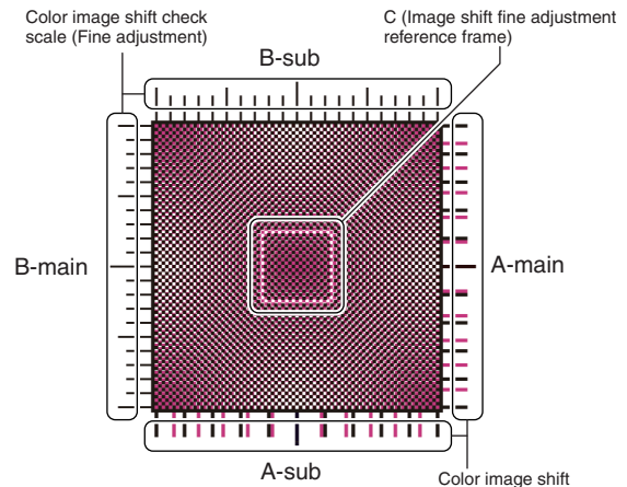
A-main: Main scan rough adjustment pattern A-sub: Sub scan rough adjustment pattern B-main: Main scan fine adjustment scale B-sub: Sub scan fine adjustment pattern C: Main scan sub scan fine adjustment pattern
